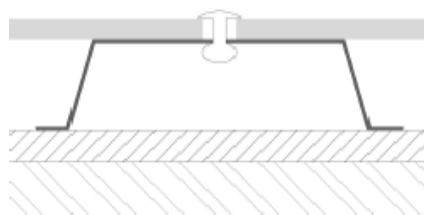
Attaching the sliding points
