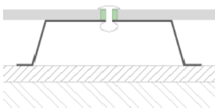
Attaching the fixed points using the fixedpoint-ring
