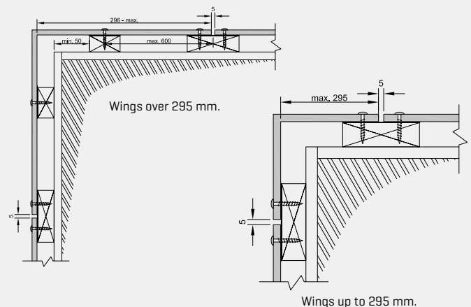
The figures show the principles for battening behind L-elements.
