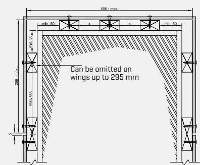
Bottom larger than 595 mm.
